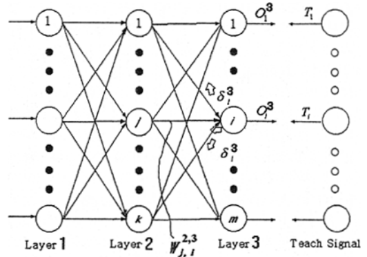
Fig. 2 3 layer neural network
