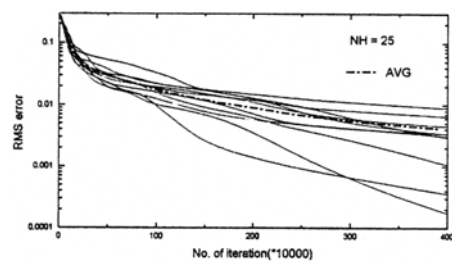
Fig. 3 Error trends when No. of neurons in hidden layer (NH) is 25
